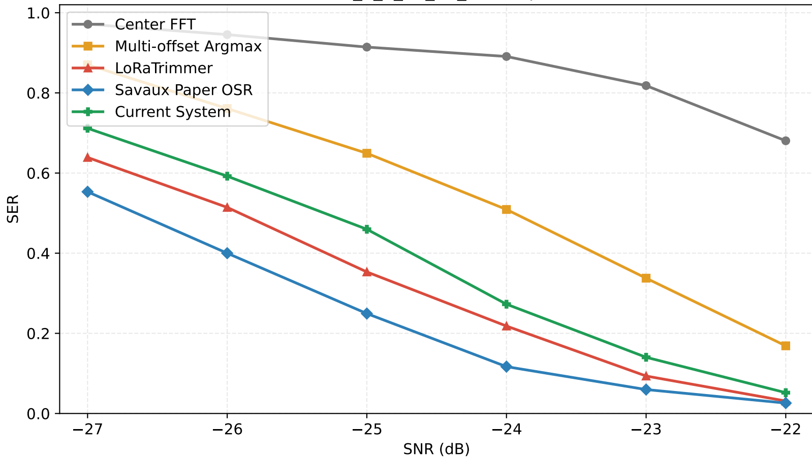
SER vs SNR (0_0_0_10_14_16, 11 packets/SNR)
